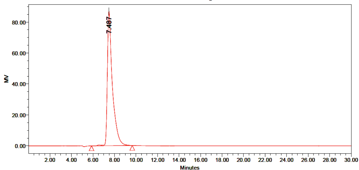
Auto-Scaled Chromatogram
