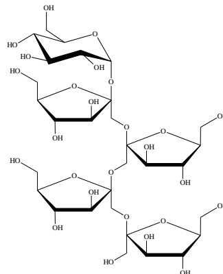
(O-β-D-Fructofuranosyl-(2-1)-β-D-fructofuranosyl-(2-1)-β-D-fructofuranosyl-(2-1)-β-D-fructofuranosyl-α-D-glucopyranose)
