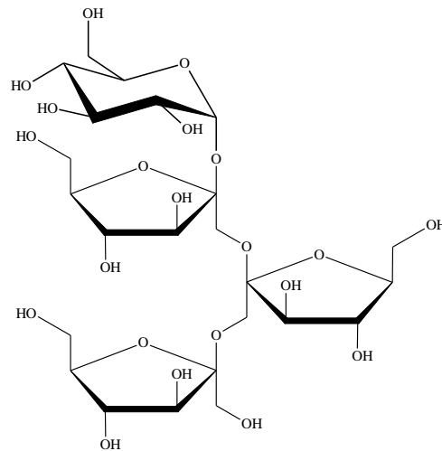
O-β-D-fructofuranosyl-(2-1)-β-D-fructofuranosyl-(2-1)-β-D-fructofuranosyl-α-D-glucopyranoside
